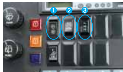
1 Clutch cut-off switch Left brake pedal can be switched between work mode for loader operations and travel mode for traveling.
